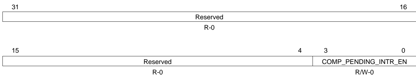
Figure 39. Receive CPPI Interrupt Enable Set Register (RCPPIENSETR)
